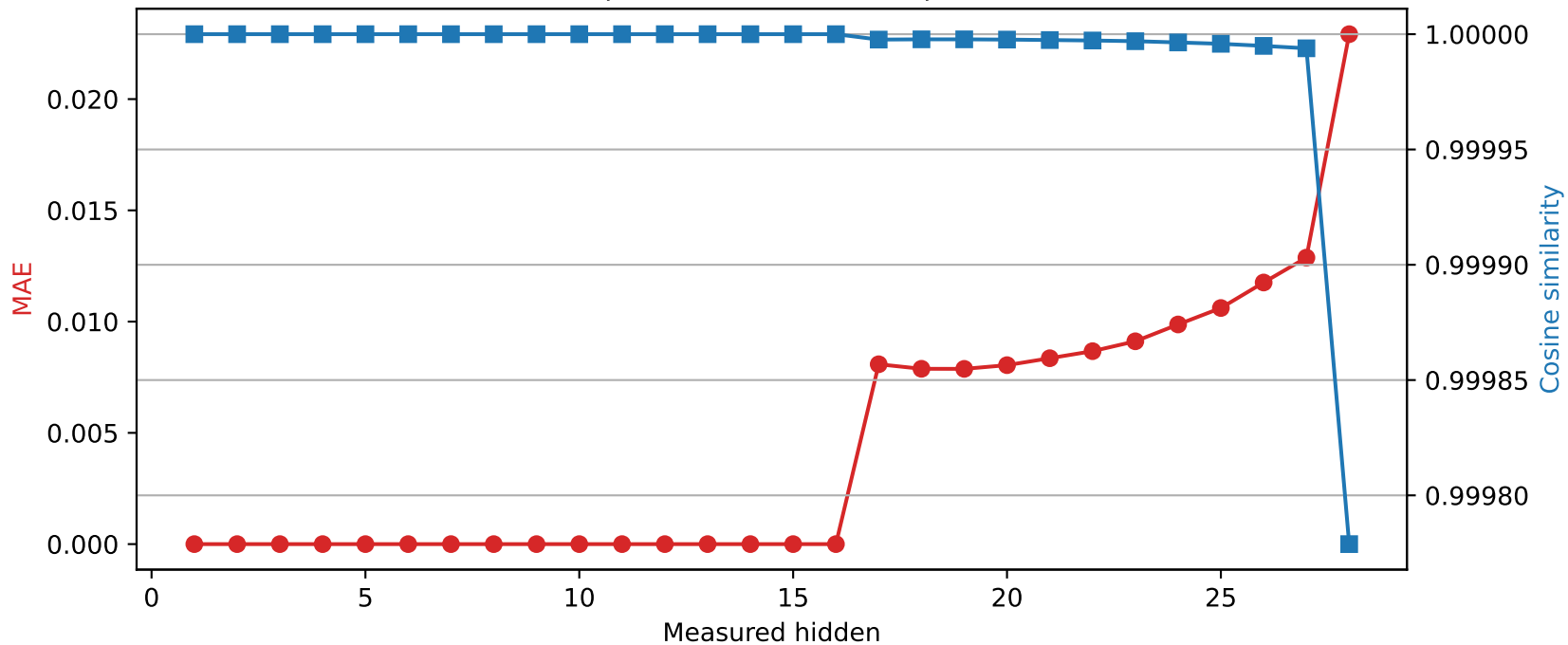
Llama-3.2-3B | Quantized layer 16 | float32 → int8
