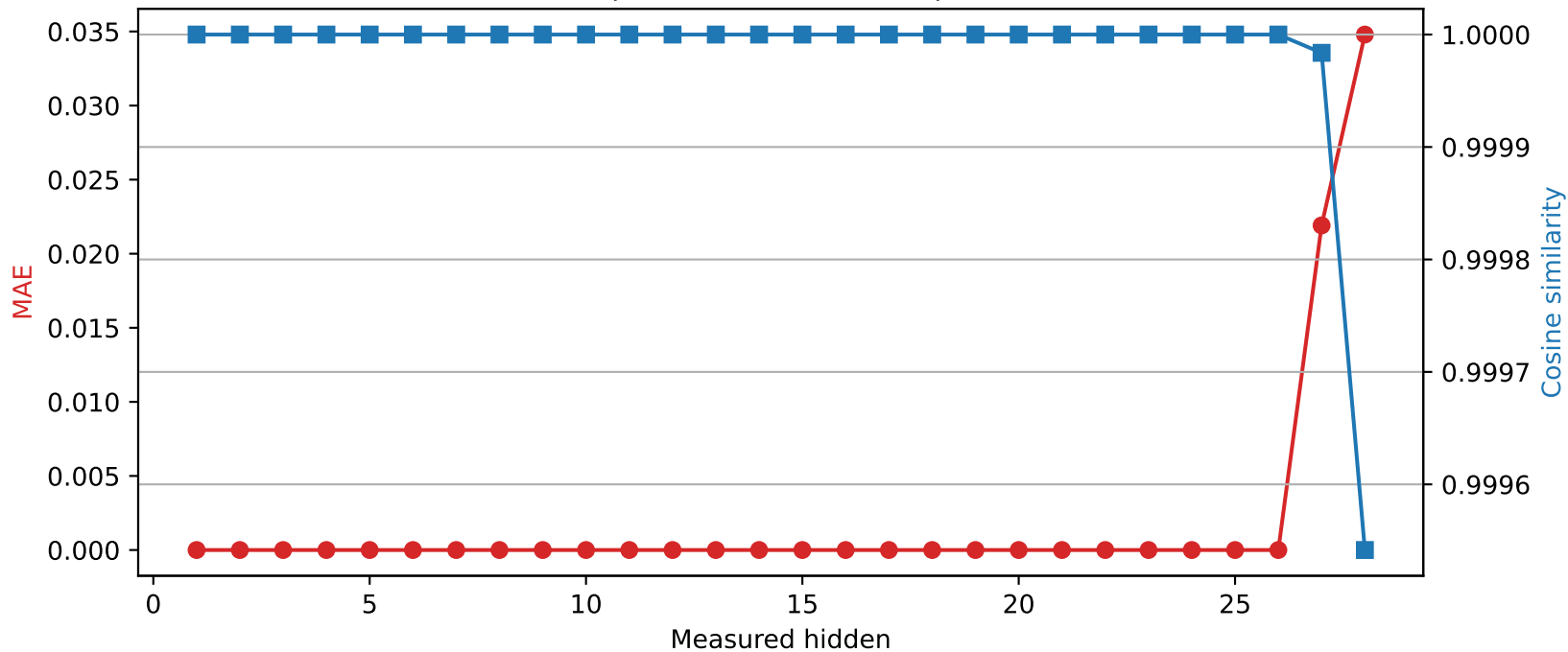
Llama-3.2-3B | Quantized layer 26 | float32 → int8
