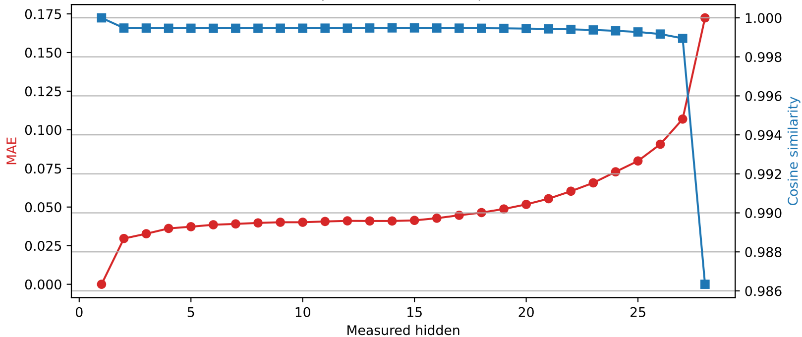
Llama-3.2-3B | Quantized layer 1 | float32 → int8
