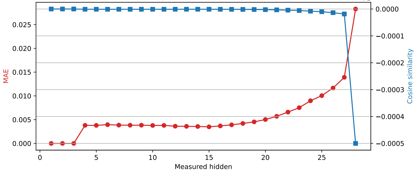
Llama-3.2-3B | Quantized layer 3 | float32 \rightarrow int8
