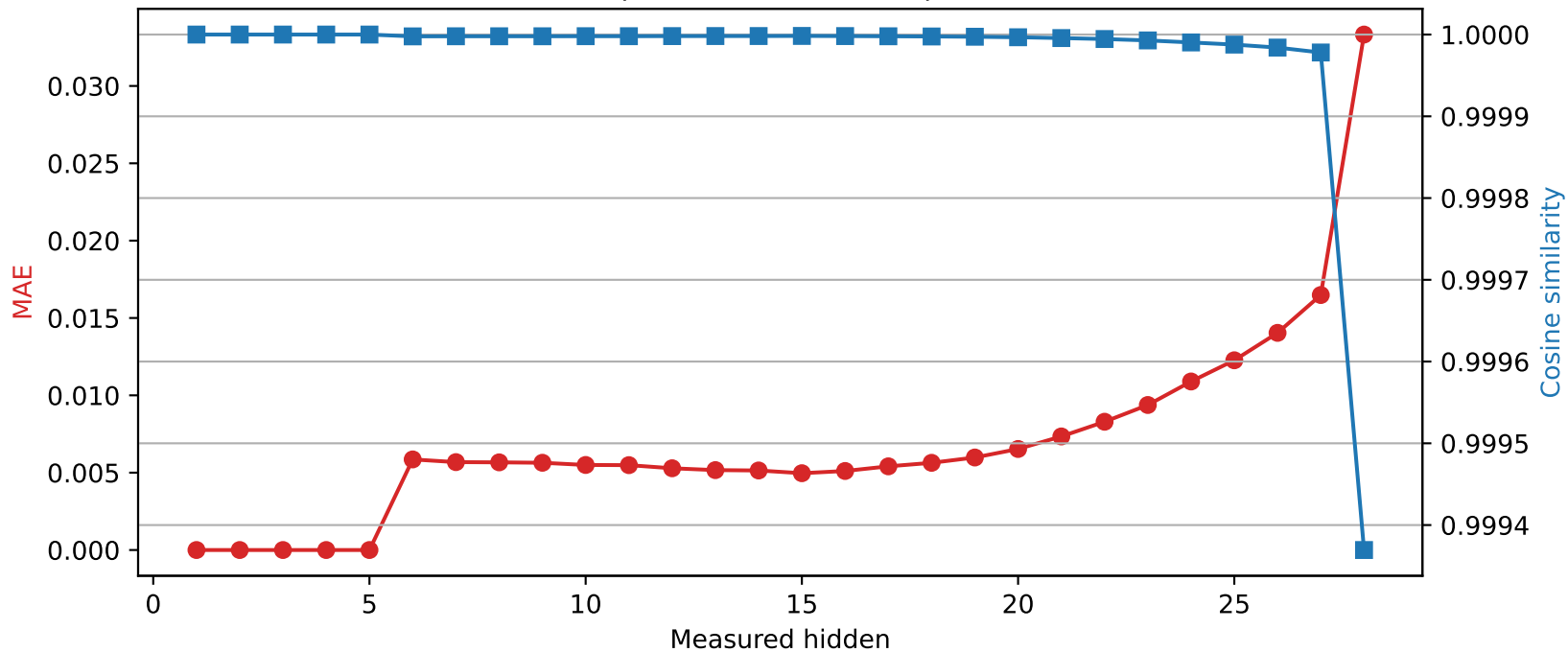
Llama-3.2-3B | Quantized layer 5 | float32 → int8
