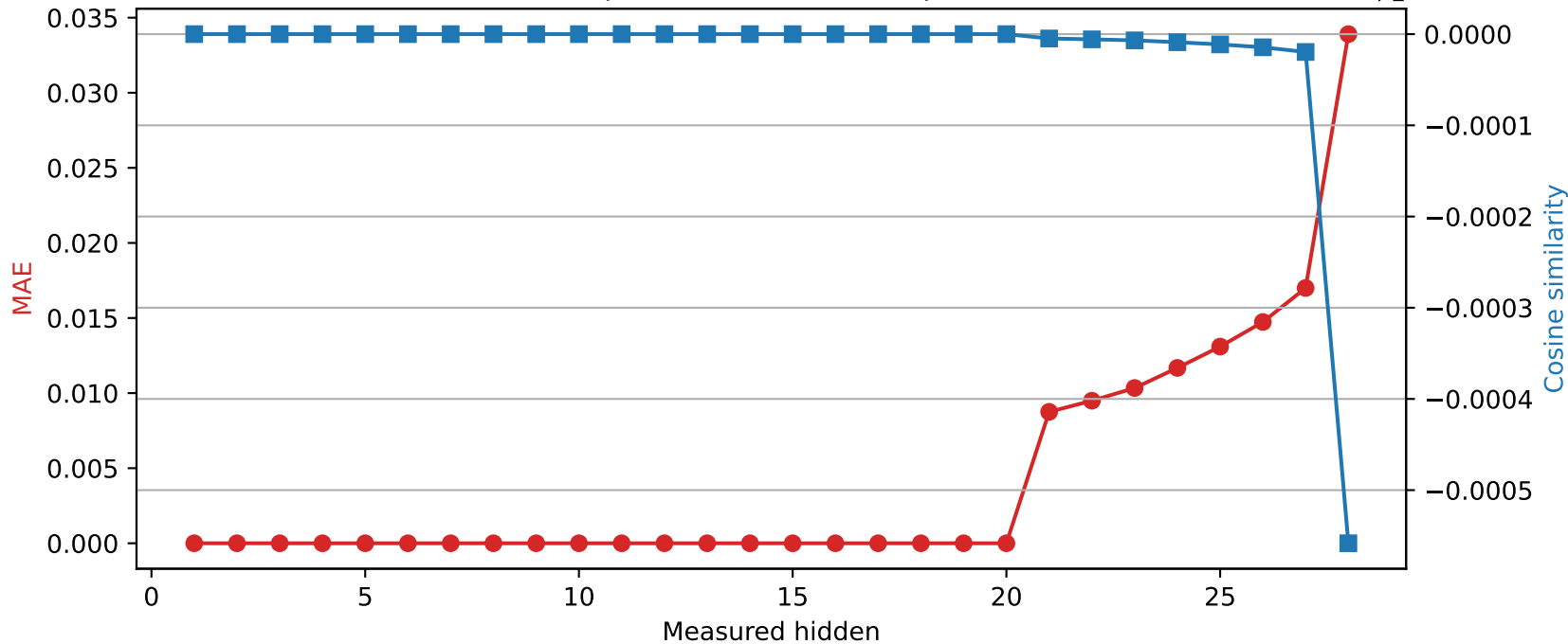
Llama-3.2-3B | Quantized layer 20 | float32 \rightarrow int8
