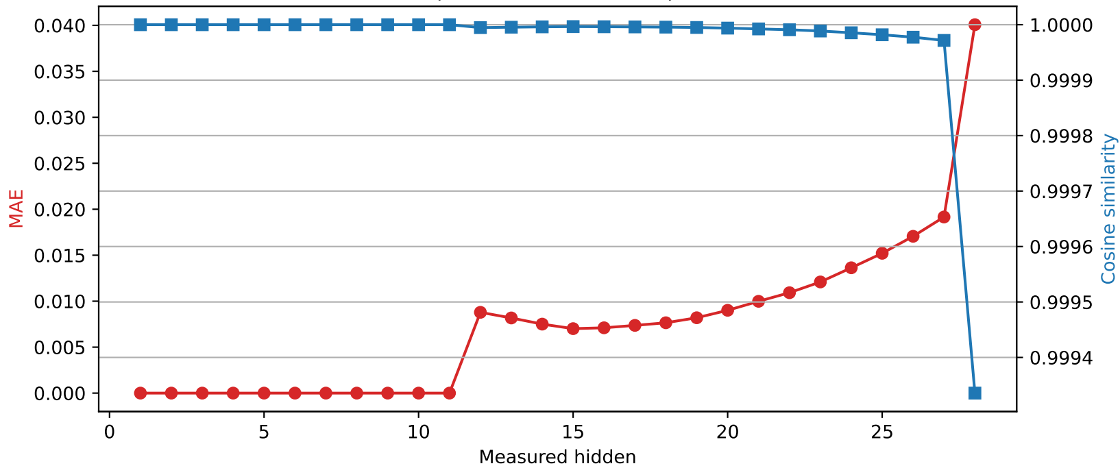
Llama-3.2-3B | Quantized layer 11 | float32 → int8
