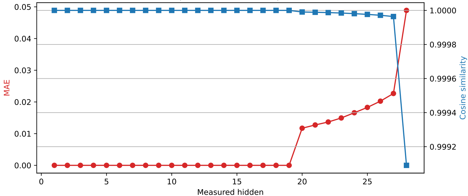
Llama-3.2-3B | Quantized layer 19 | float32 → int8
