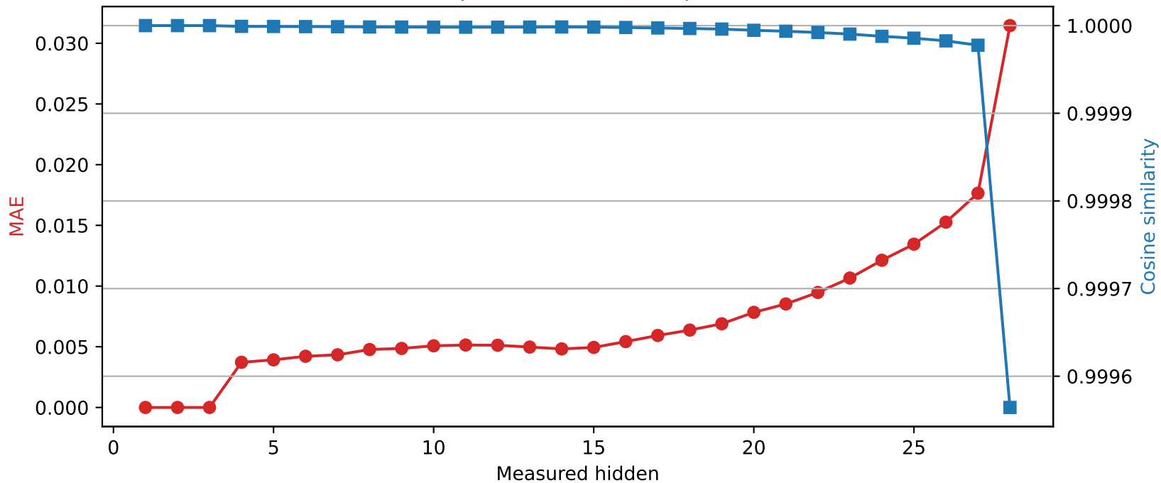
Llama-3.2-3B | Quantized layer 3 | float32 → int8
