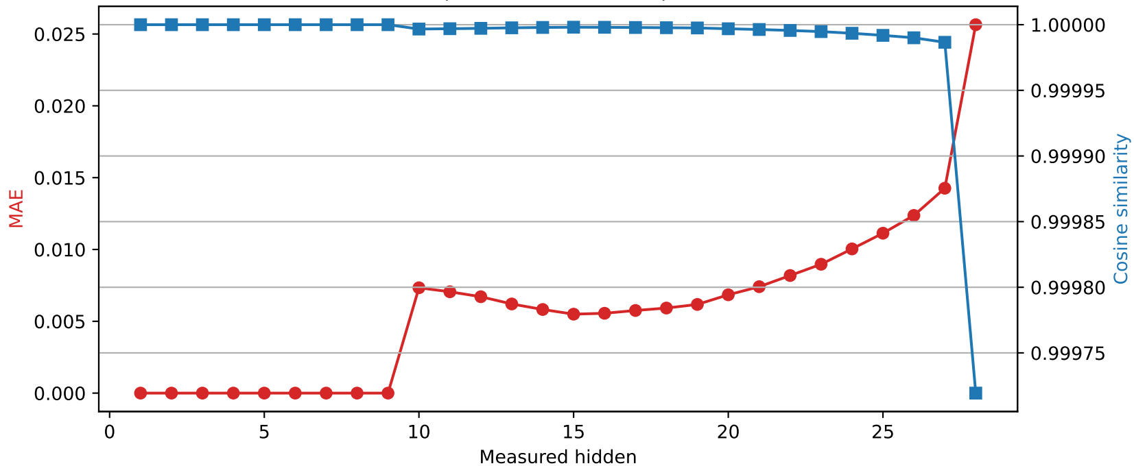
Llama-3.2-3B | Quantized layer 9 | float32 → int8
