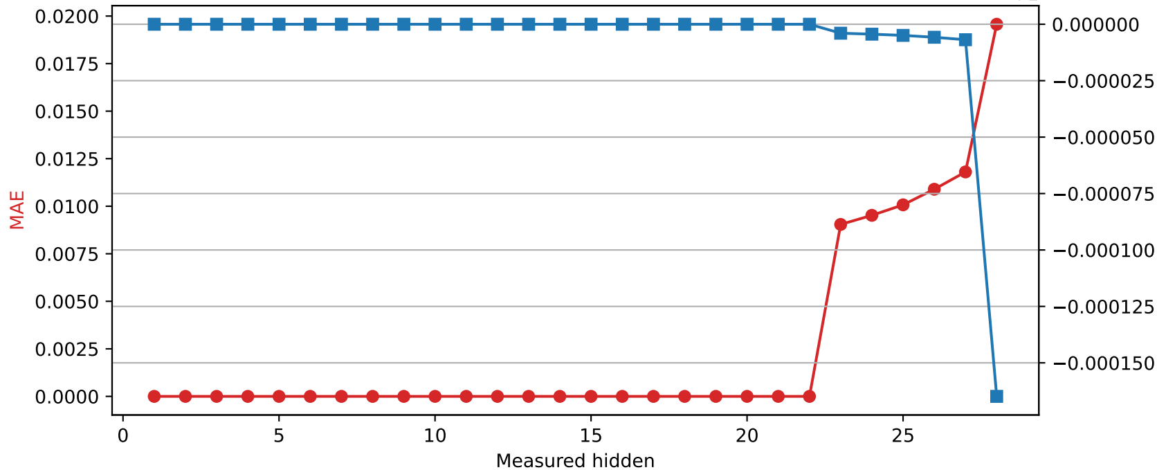
Llama-3.2-3B | Quantized layer 22 | float32 → int8
