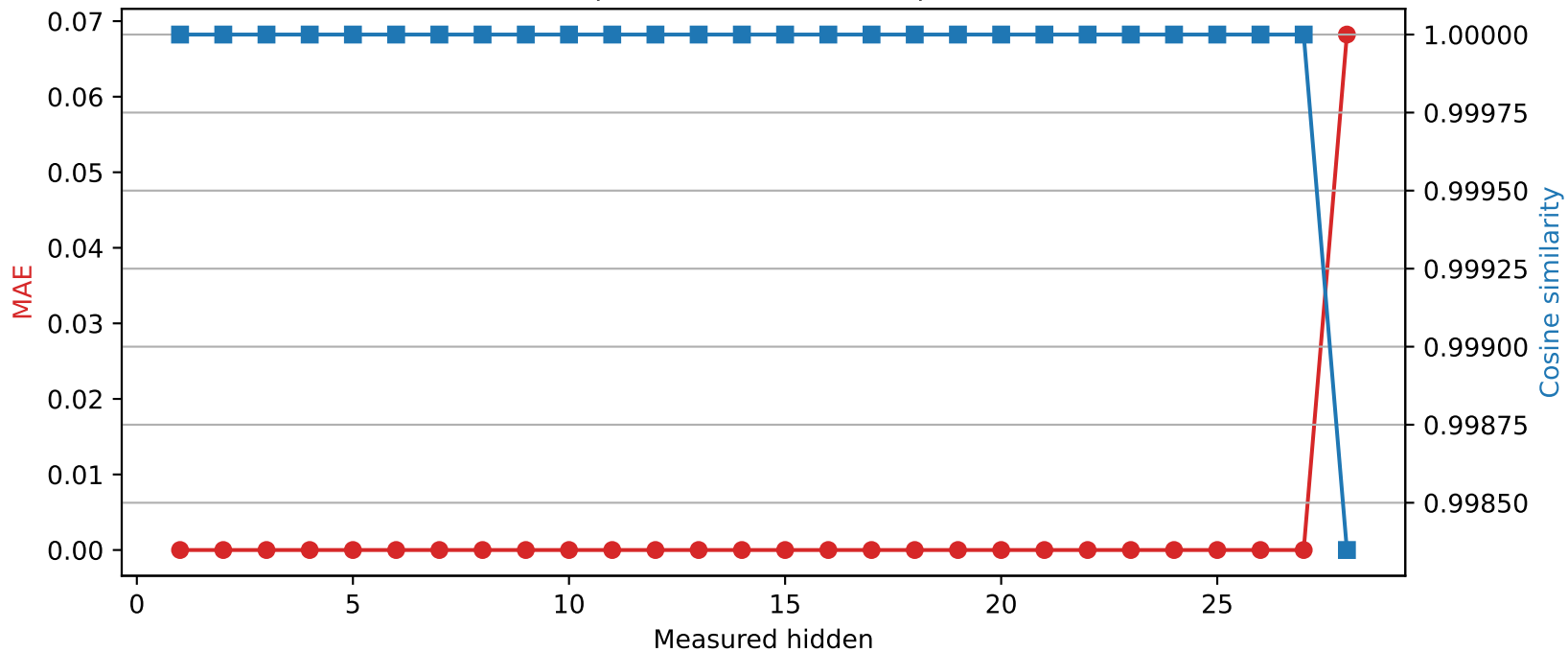
Llama-3.2-3B | Quantized layer 27 | float32 \rightarrow int8
