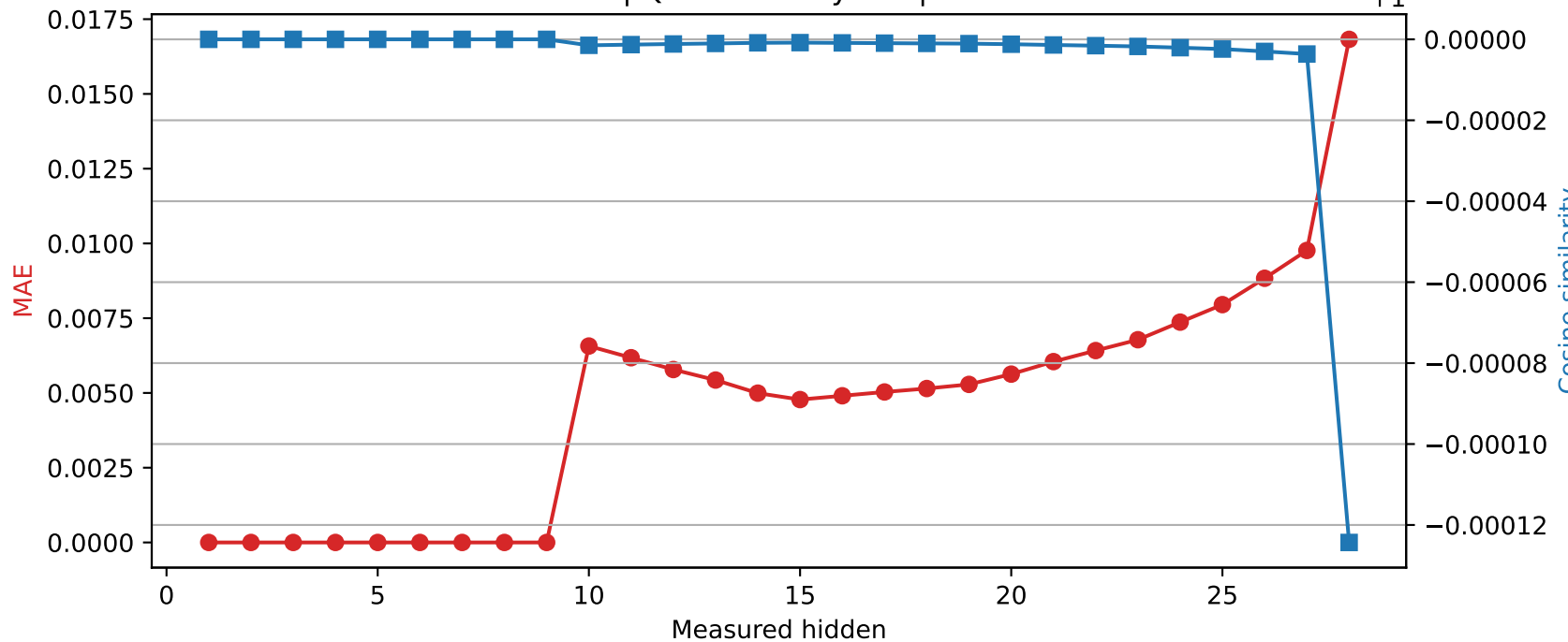
Llama-3.2-3B | Quantized layer 9 | float64 → int8
