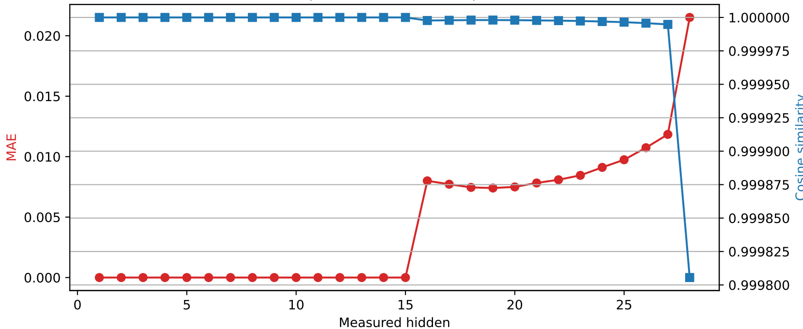
Llama-3.2-3B | Quantized layer 15 | float64 → int8
