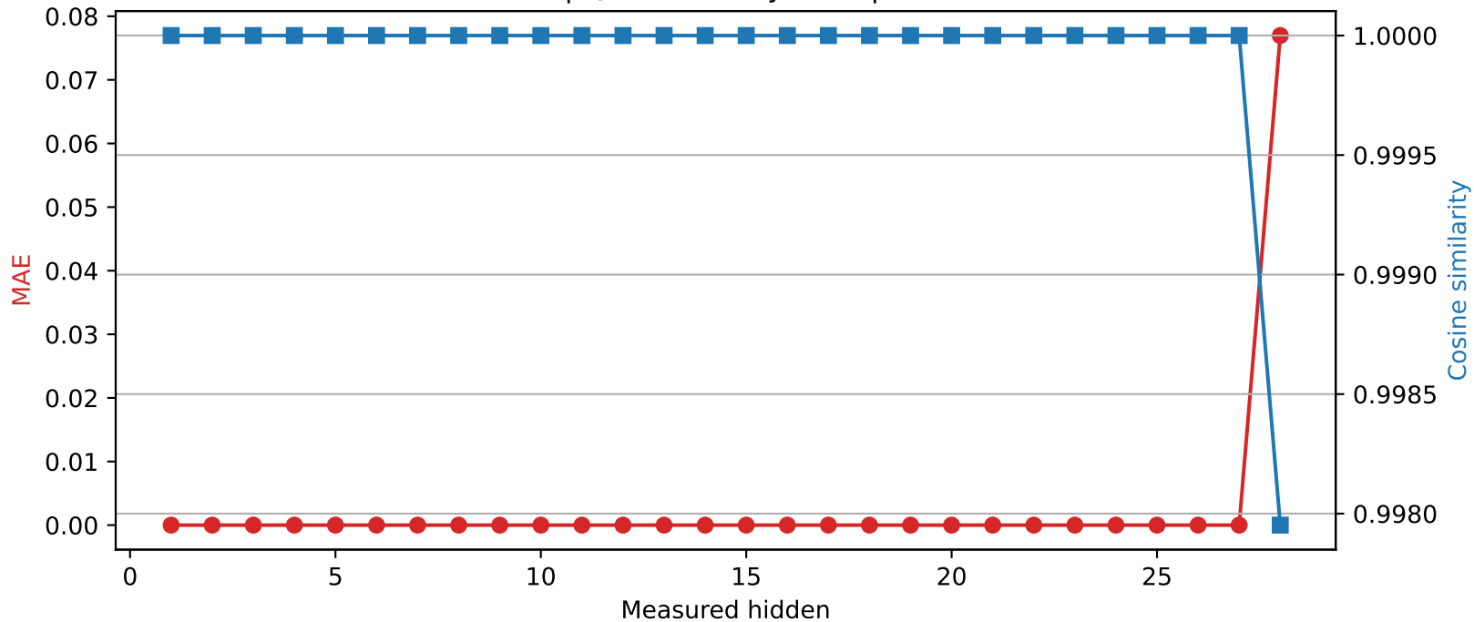
Llama-3.2-3B | Quantized layer 27 | float64 → int8
