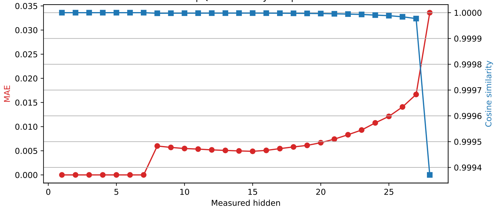
Llama-3.2-3B | Quantized layer 7 | float64 → int8
