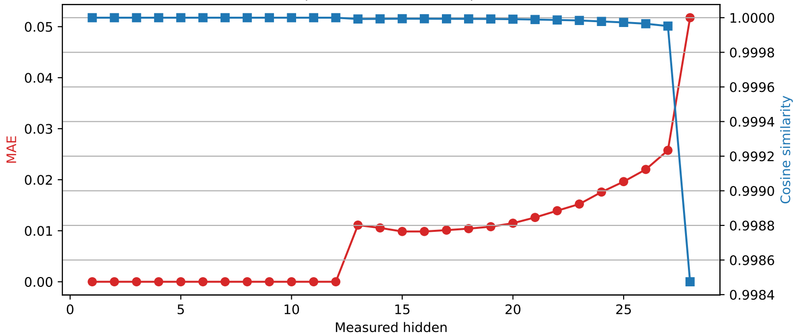
Llama-3.2-3B | Quantized layer 12 | float64 → int8
