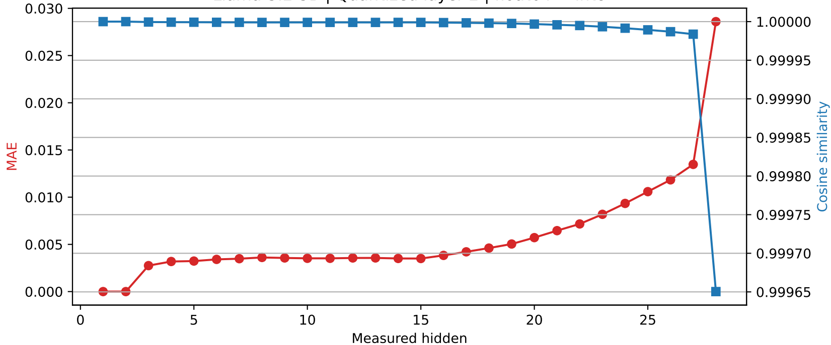
Llama-3.2-3B | Quantized layer 2 | float64 → int8
