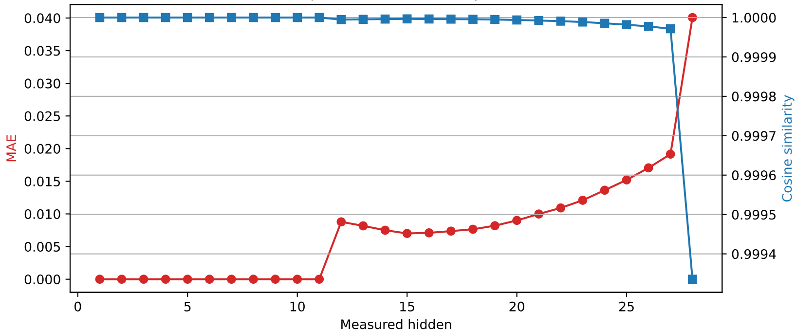
Llama-3.2-3B | Quantized layer 11 | float64 → int8
