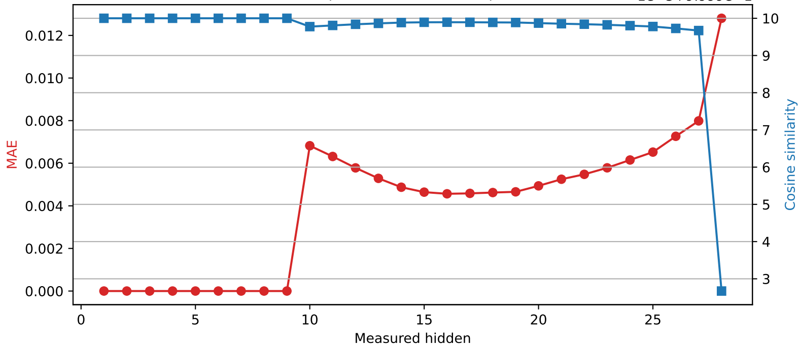
Llama-3.2-3B | Quantized layer 9 | float64 → int8
