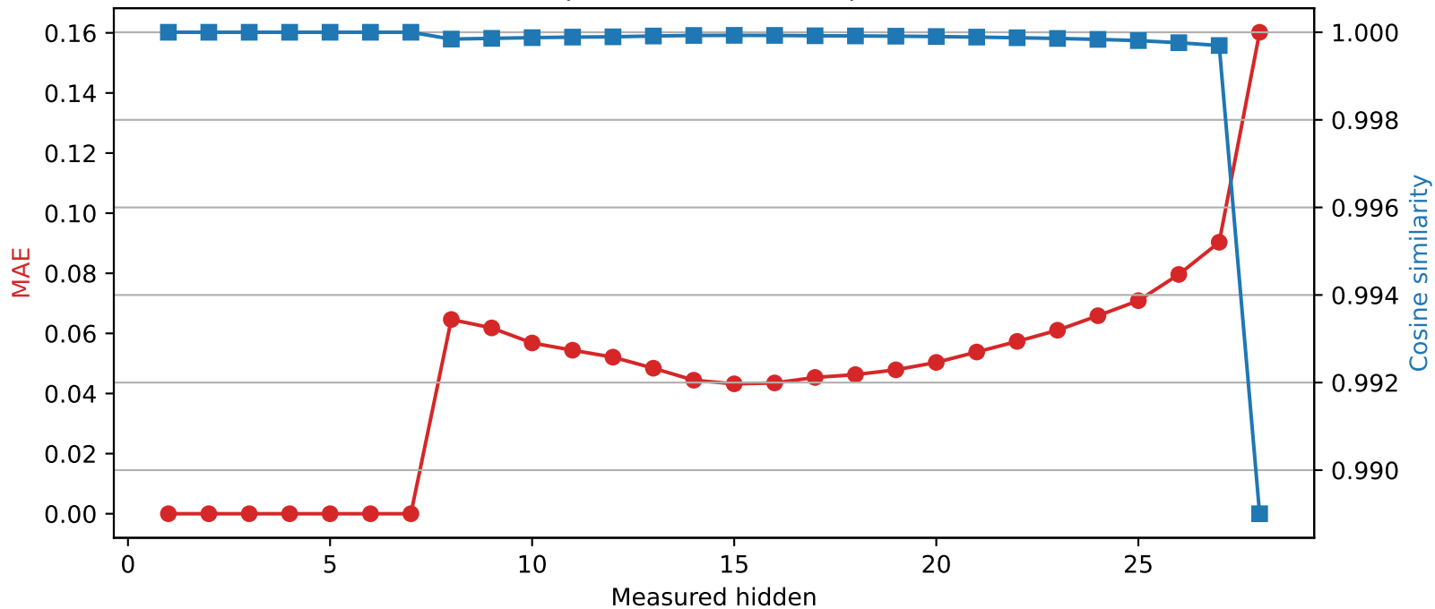
Llama-3.2-3B | Quantized layer 7 | float16 → int4
