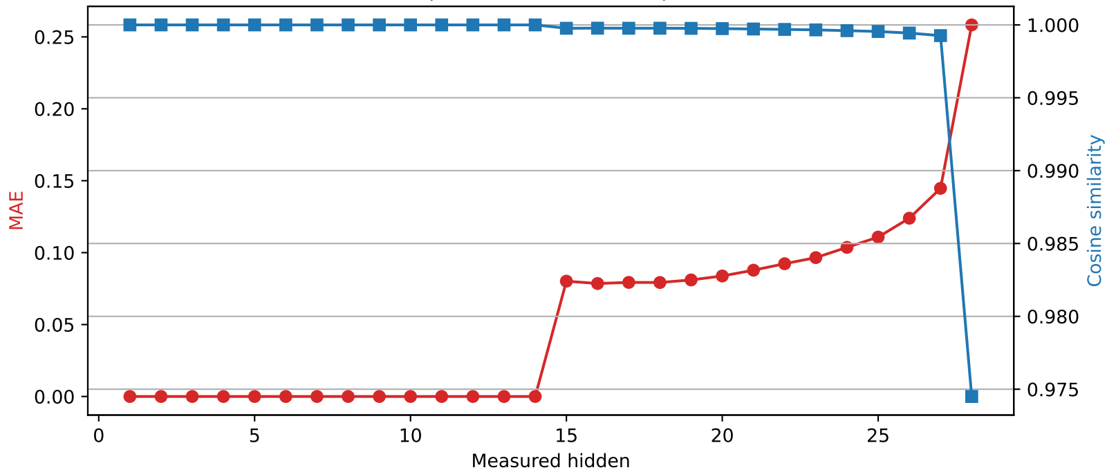
Llama-3.2-3B | Quantized layer 14 | float16 \rightarrow int4
