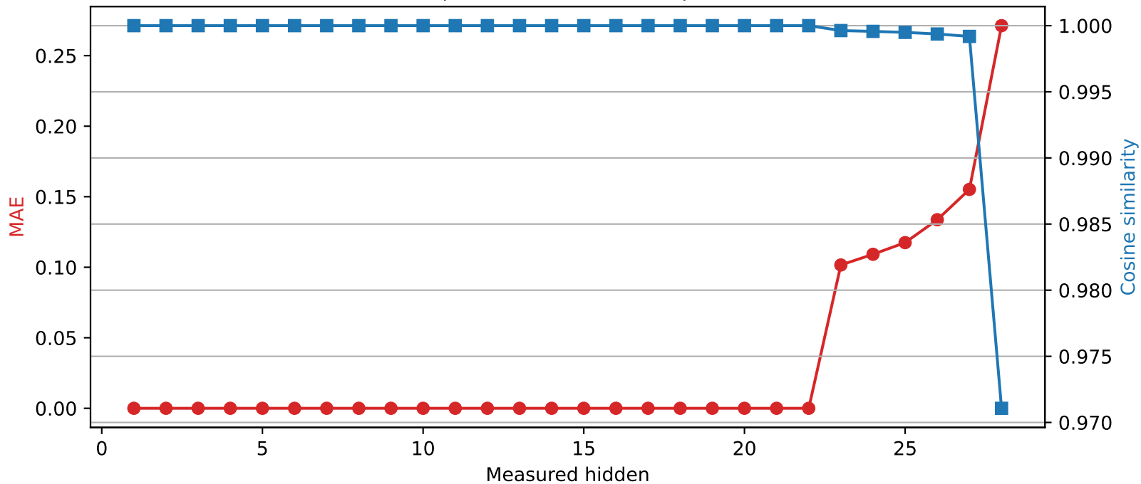
Llama-3.2-3B | Quantized layer 22 | float16 \rightarrow int4
