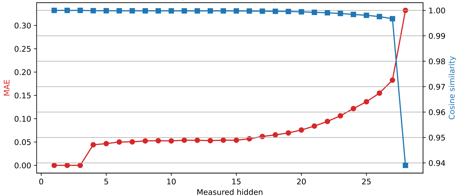
Llama-3.2-3B | Quantized layer 3 | float16 \rightarrow int4
