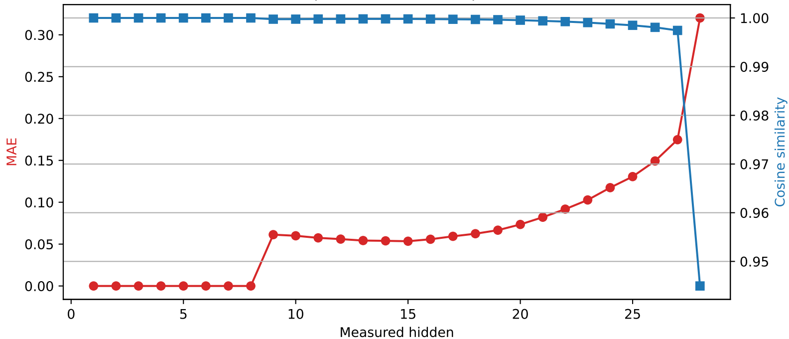
Llama-3.2-3B | Quantized layer 8 | float16 \rightarrow int4
