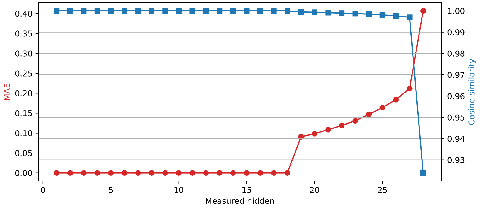
Llama-3.2-3B | Quantized layer 18 | float16 → int4
