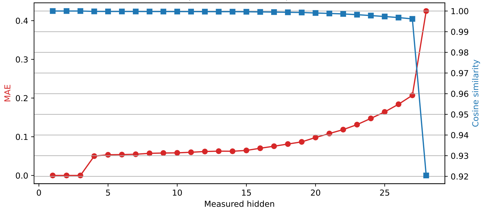
Llama-3.2-3B | Quantized layer 3 | float16 → int4
