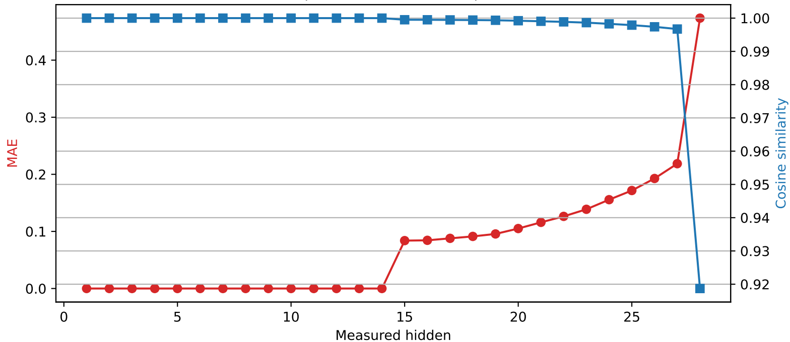
Llama-3.2-3B | Quantized layer 14 | float16 → int4
