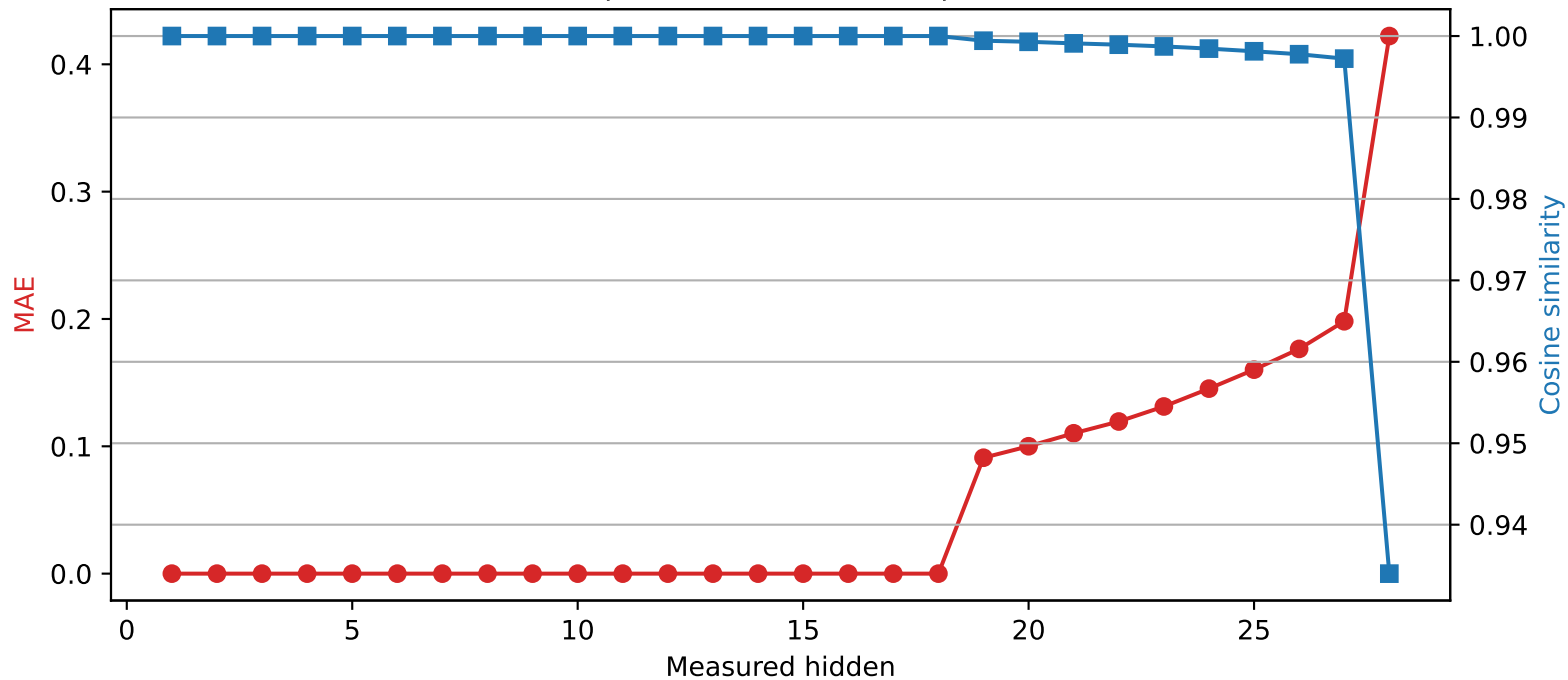
Llama-3.2-3B | Quantized layer 18 | float16 \rightarrow int4
