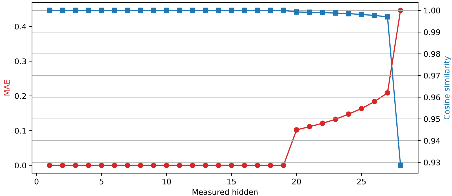
Llama-3.2-3B | Quantized layer 19 | float16 → int4
