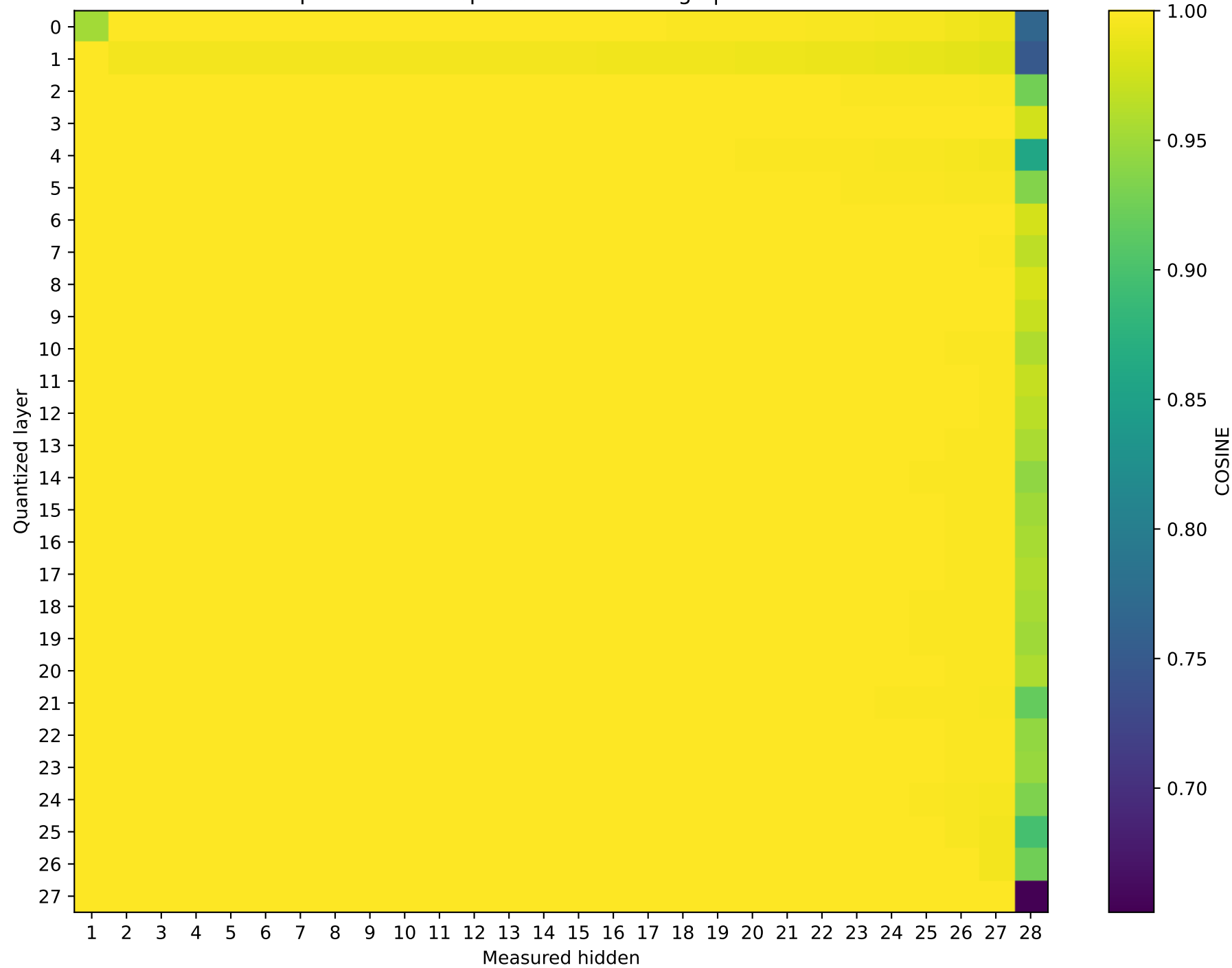
Llama-3.2-3B Prompt 3: cos sim representation damage | float16 → int4
