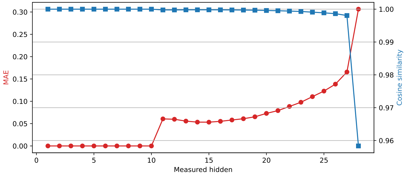
Llama-3.2-3B | Quantized layer 10 | float16 \rightarrow int4
