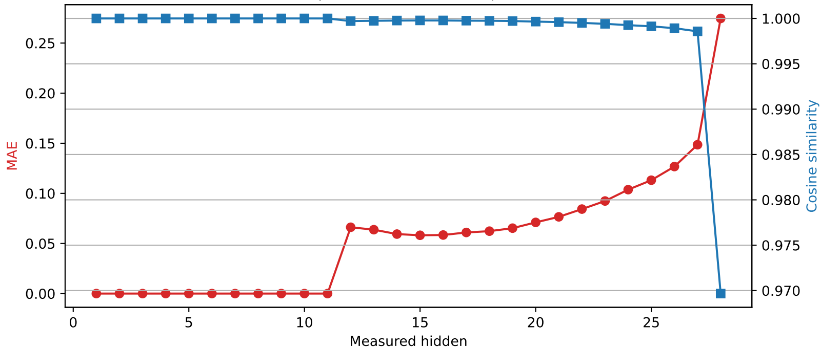
Llama-3.2-3B | Quantized layer 11 | float16 → int4
