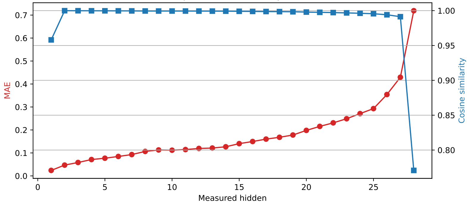
Llama-3.2-3B | Quantized layer 0 | float16 → int4
