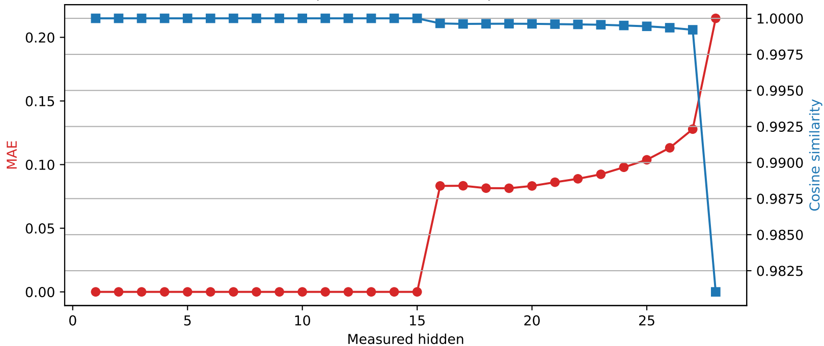
Llama-3.2-3B | Quantized layer 15 | float16 → int4
