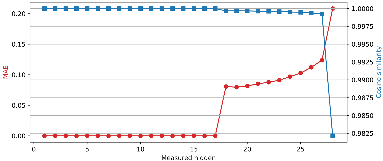
Llama-3.2-3B | Quantized layer 17 | float16 → int4
