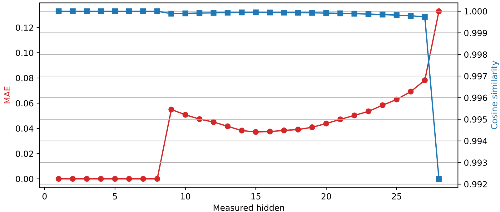
Llama-3.2-3B | Quantized layer 8 | float32 \rightarrow int4
