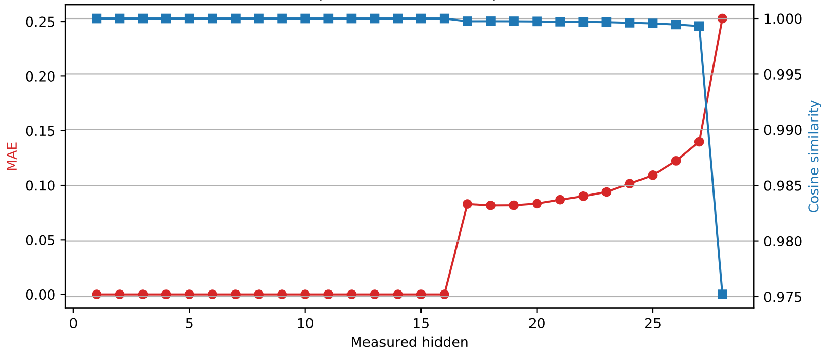
Llama-3.2-3B | Quantized layer 16 | float32 → int4
