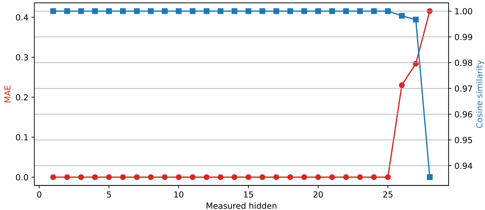
Llama-3.2-3B | Quantized layer 25 | float32 → int4
