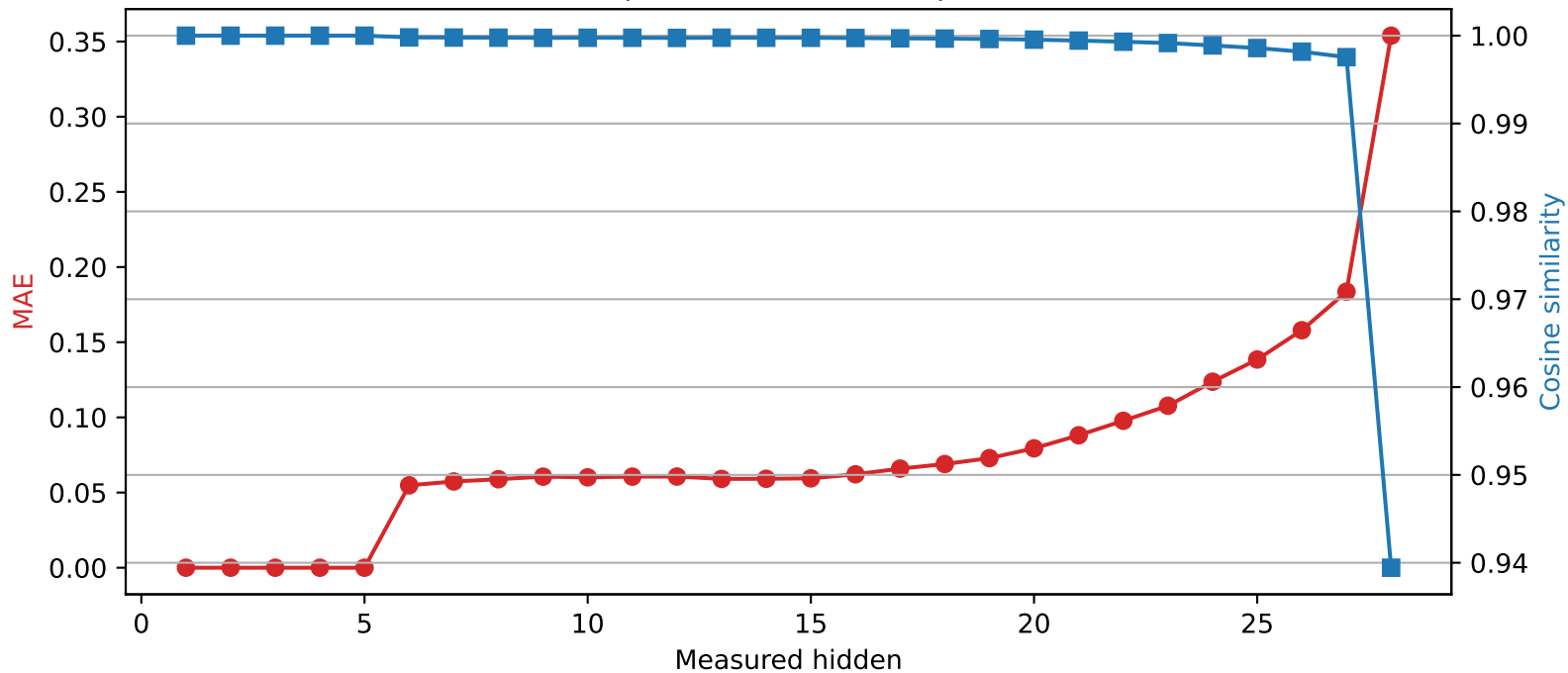
Llama-3.2-3B | Quantized layer 5 | float32 → int4
