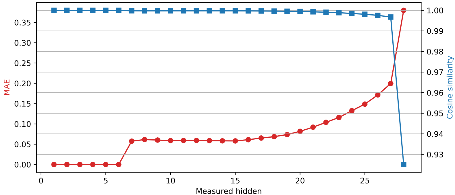
Llama-3.2-3B | Quantized layer 6 | float32 \rightarrow int4
