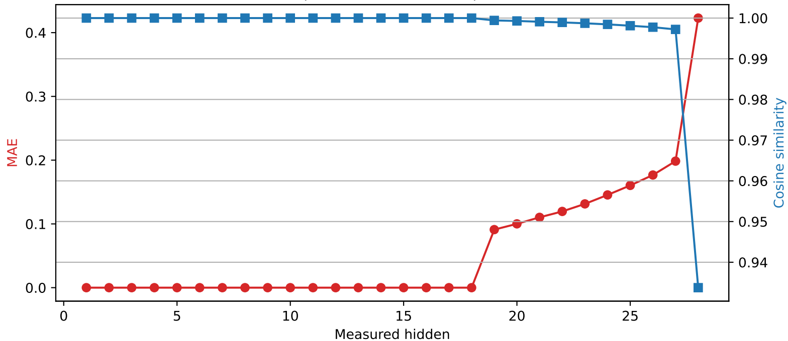
Llama-3.2-3B | Quantized layer 18 | float32 \rightarrow int4
