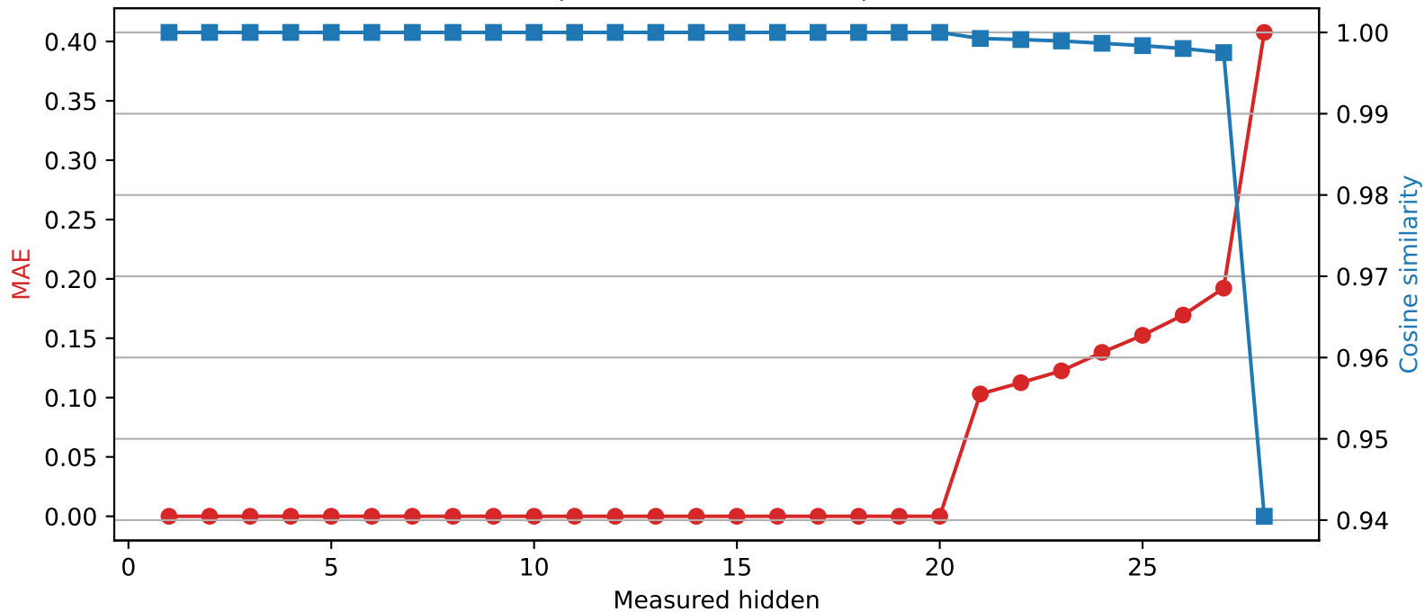
Llama-3.2-3B | Quantized layer 20 | float32 → int4
