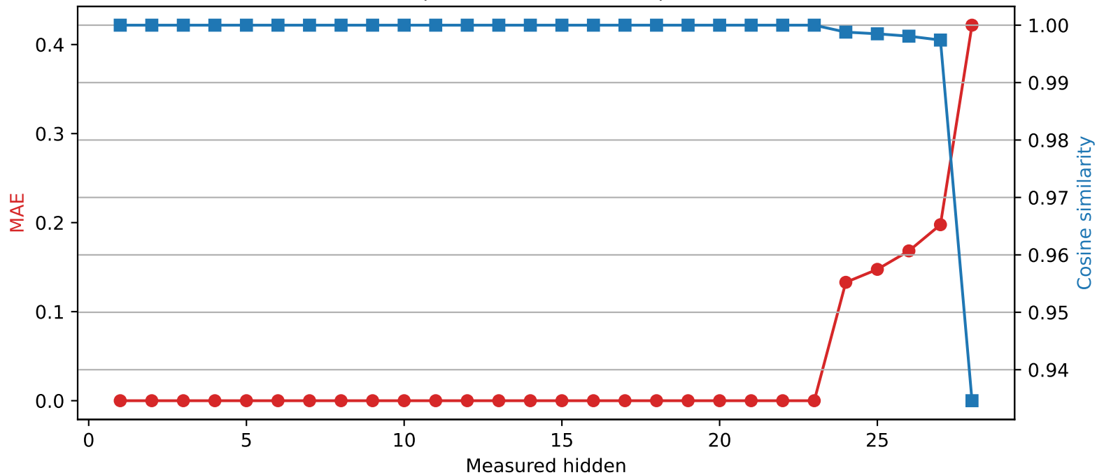
Llama-3.2-3B | Quantized layer 23 | float32 → int4
