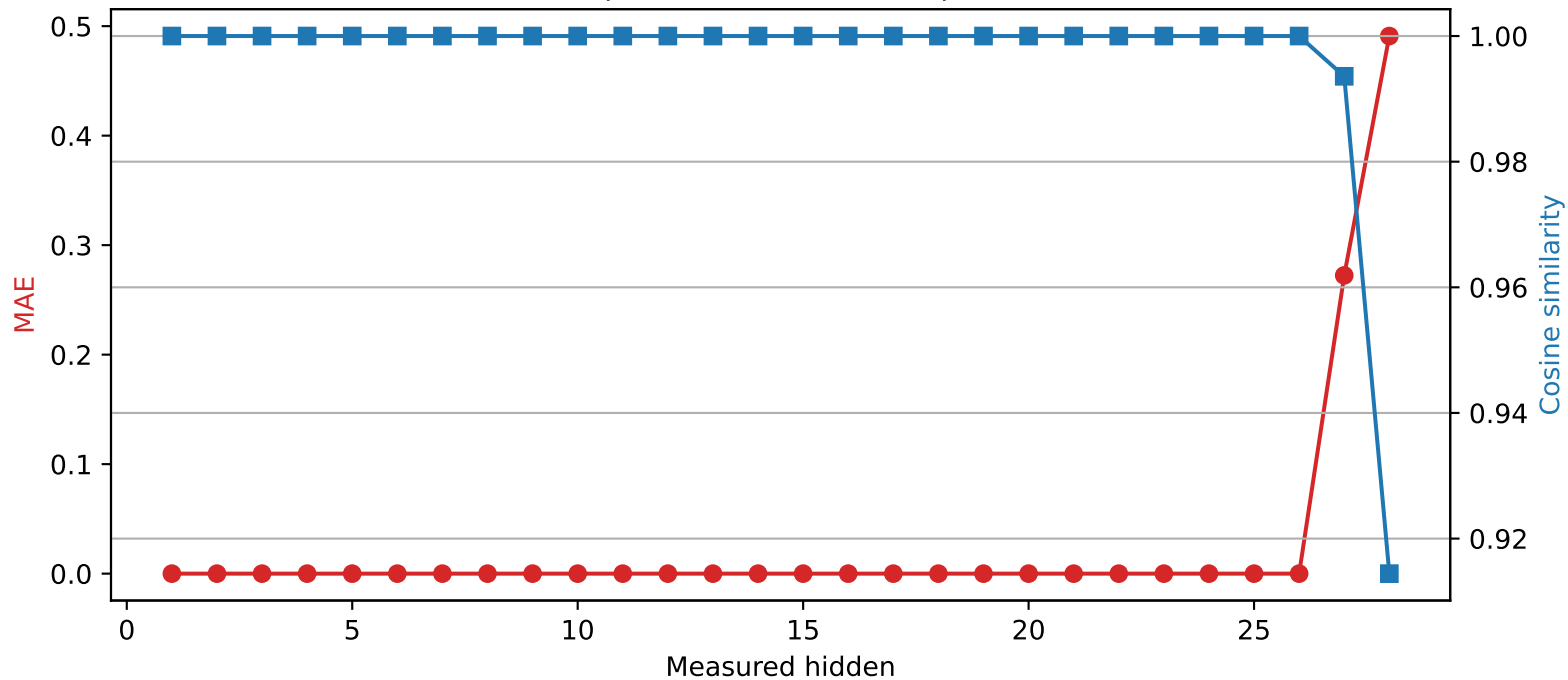
Llama-3.2-3B | Quantized layer 26 | float32 → int4
