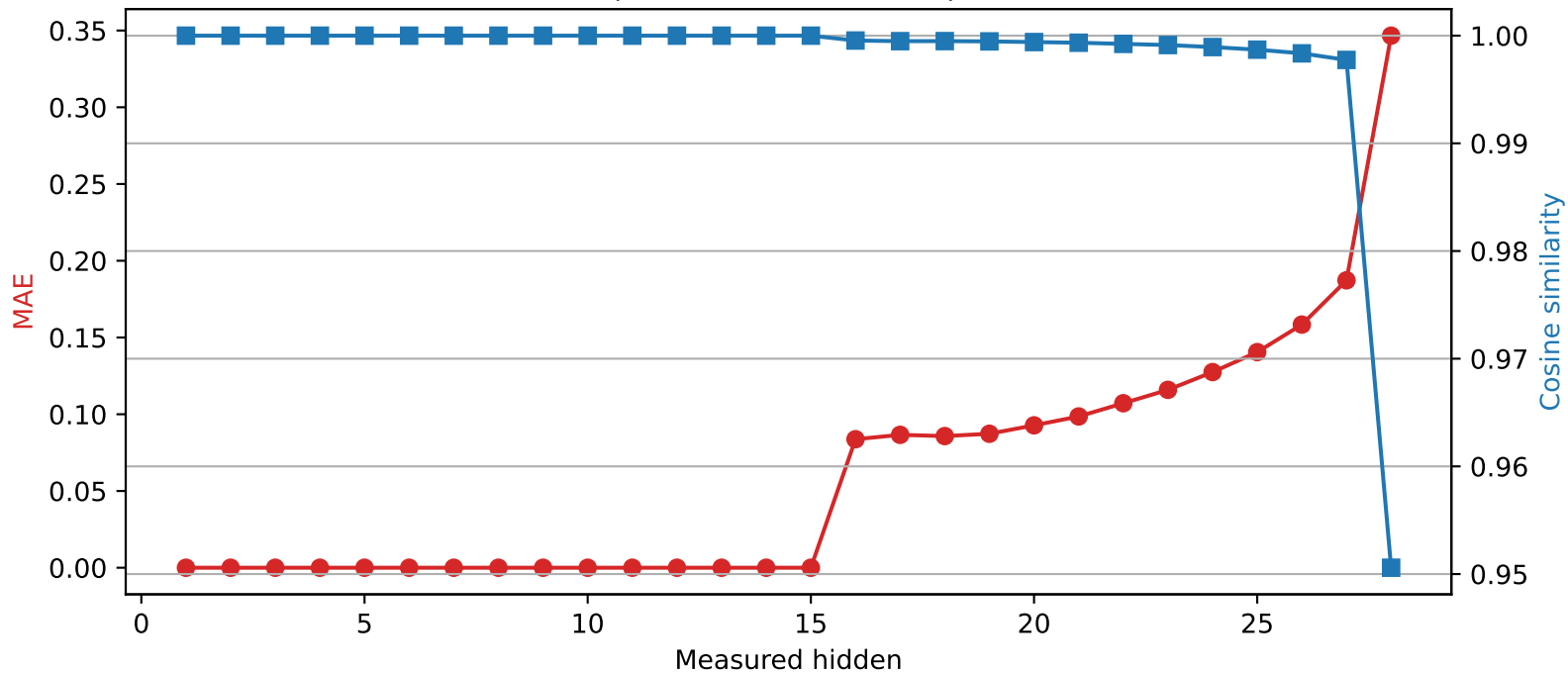
Llama-3.2-3B | Quantized layer 15 | float32 → int4
