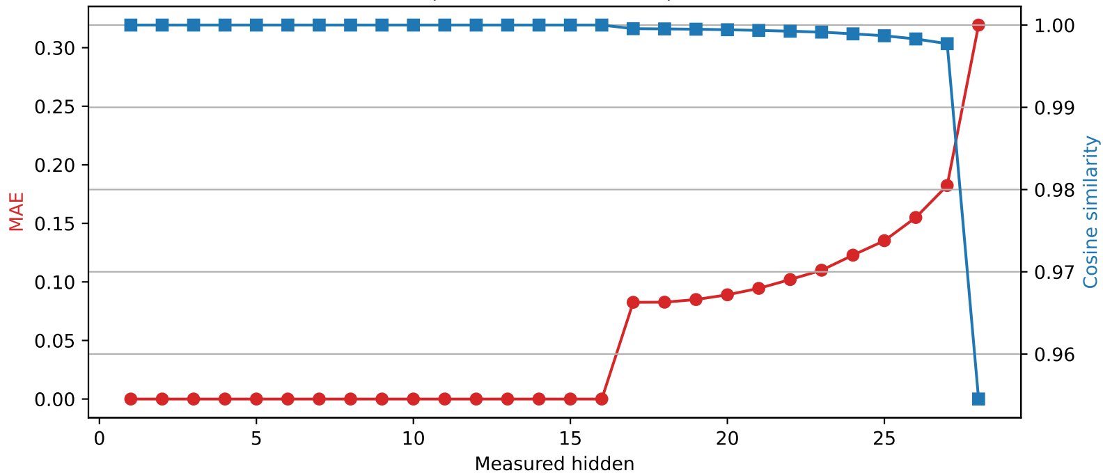
Llama-3.2-3B | Quantized layer 16 | float32 \rightarrow int4
