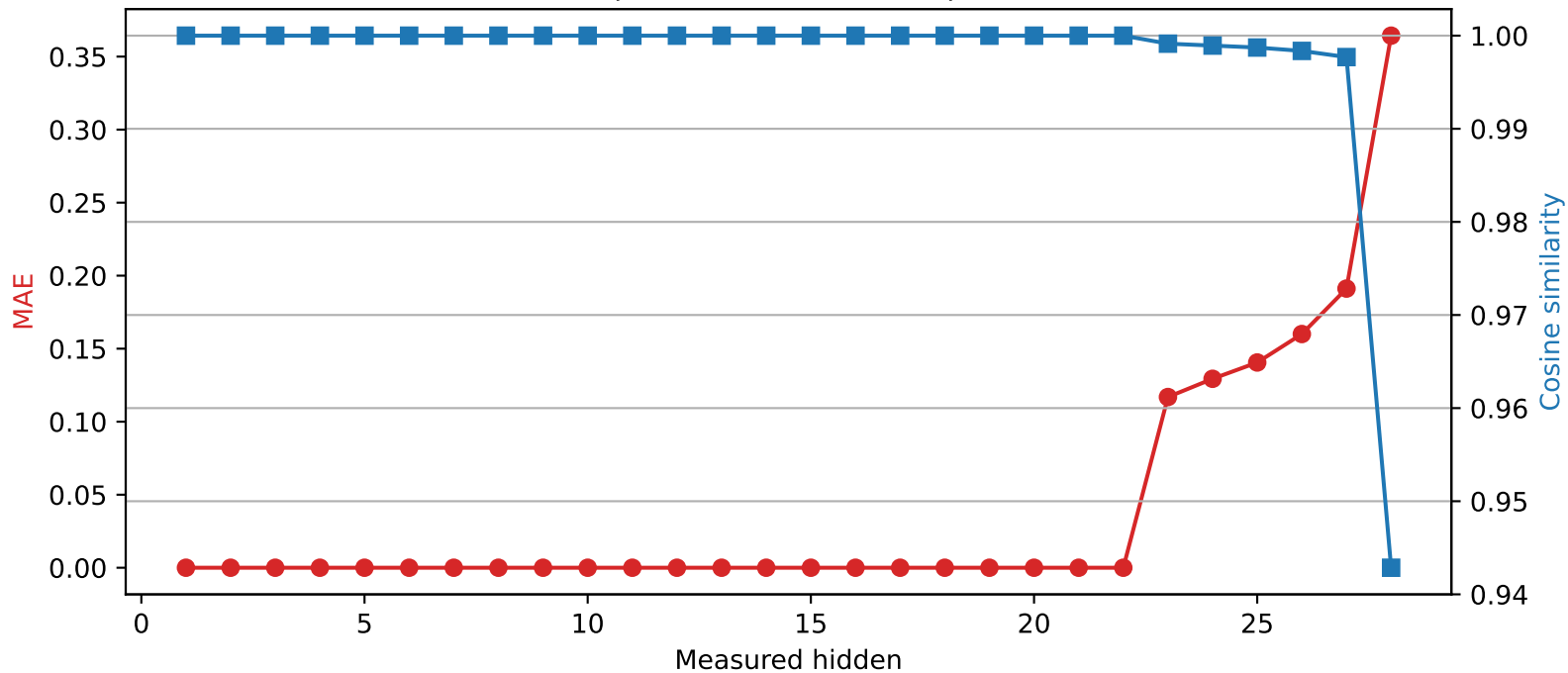
Llama-3.2-3B | Quantized layer 22 | float32 → int4
