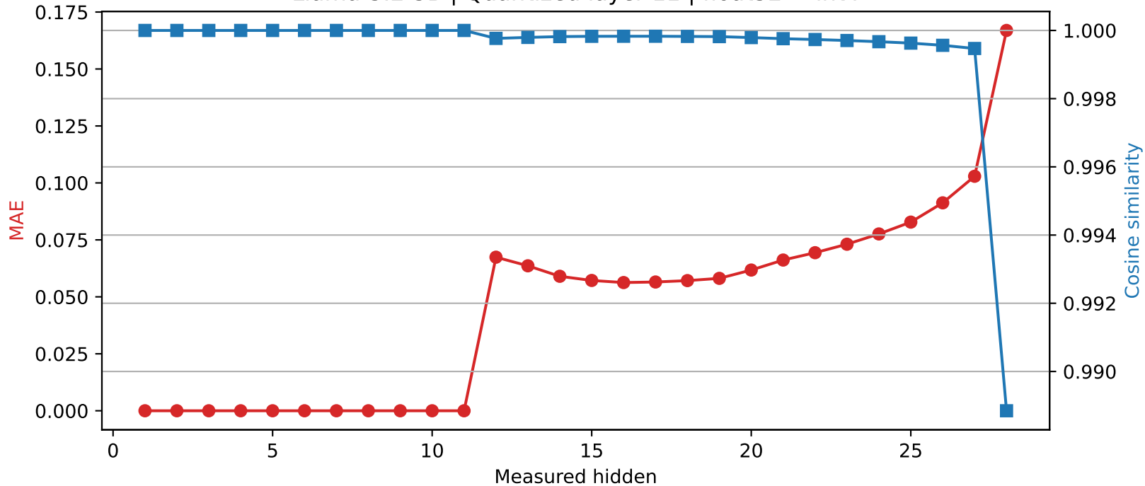
Llama-3.2-3B | Quantized layer 11 | float32 \rightarrow int4
