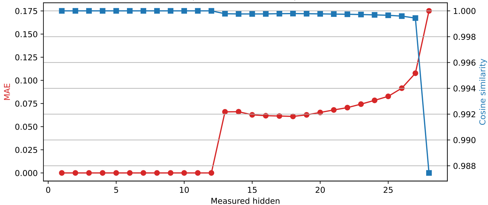
Llama-3.2-3B | Quantized layer 12 | float32 → int4
